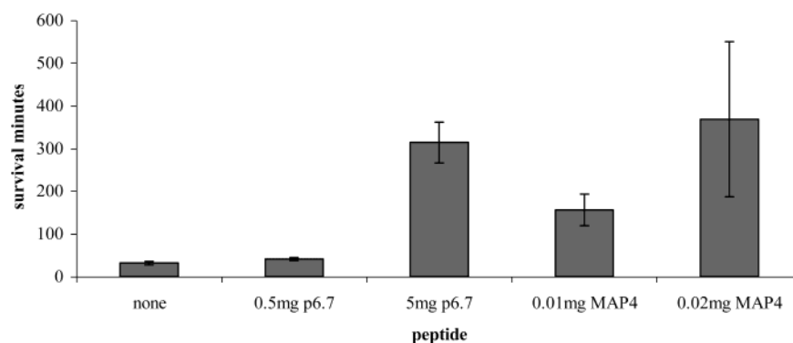
FIGURE 4: In vivo activity of MAP4p6.7 and p6.7. 15 g Swiss mice were injected subcutaneously with 10 \mu g/100 \mu L of \alpha -bgt. After 5 min they were injected s.c. with 250 \mu L of MAP4p6.7 or p6.7. The average survival time after injection of toxin was calculated with one group of 30 mice. Results of mice treated with 20 \mu g MAP4p6.7 are from nine mice, while the others are from groups of three mice. The results obtained with MAP4p6.7 doses affording protection are reported in Table 2.
