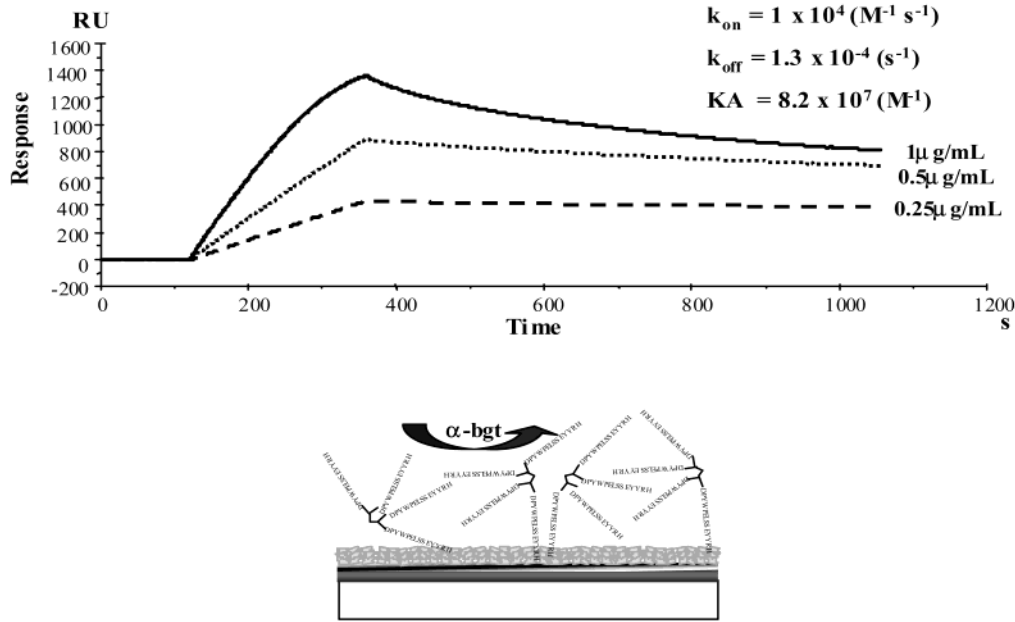
FIGURE 1: BIAcore kinetic analysis of \alpha -bgt binding to immobilized MAP4p6.7. \alpha -bgt, from 0.25 to 1 \mu g/mL, was injected with a flow of 30 \mu L/min onto a CM5 sensor chip where MAP4p6.7 had been covalently bound by standard amine coupling. Association and dissociation kinetic rates were calculated by the BIAevaluation 3.0 program. A schematic representation of the experiment is shown under the sensorgram: \alpha -bgt was injected on a CM5 sensor chip prepared with covalently bound MAP4p6.7.
